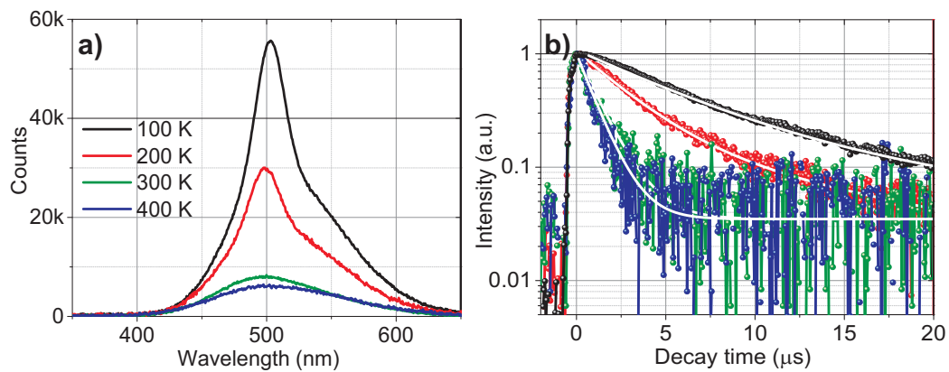
Fig. S6. Temperature dependent a) PL spectra and b) Time-Resolved PL (TRPL) decay curves of (\text{C}_6\text{H}_5\text{CH}_2\text{NH}_3)_2\text{SnBr}_4 recorded from 100 to 400 K with an interval 100 K. The excitation wavelength is 266 nm while for the decay curves, the monitoring wavelength is 500 nm. The white lines in b) are the exponential fits of the curves. The lifetimes at 100, 200, 300, and 400 K are 8.75, 4.59, 1.05, and 1.01 \mu\text{s} , respectively.
