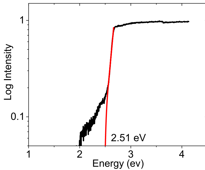
Fig. S5. The optical bandgap determined through the Tauc plot of absorption spectra of (\text{C}_6\text{H}_5\text{CH}_2\text{NH}_3)_2\text{SnBr}_4 .
