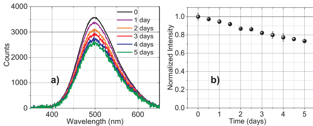
Fig. S4. a) Photoluminescence (PL) spectra and b) PL intensity as function of air exposure day of (\text{C}_6\text{H}_5\text{CH}_2\text{NH}_3)_2\text{SnBr}_4 for 5 days. The excitation is at 266 nm with 30 kHz picosecond pulsed diode laser.
