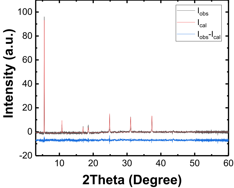
Fig. S1. Experimental I_{obs} and simulated I_{cal} XRD patterns of (C_6H_5CH_2NH_3)_2SnBr_4 . The difference between the simulated and the experimental peaks is denoted I_{obs} - I_{cal} .
