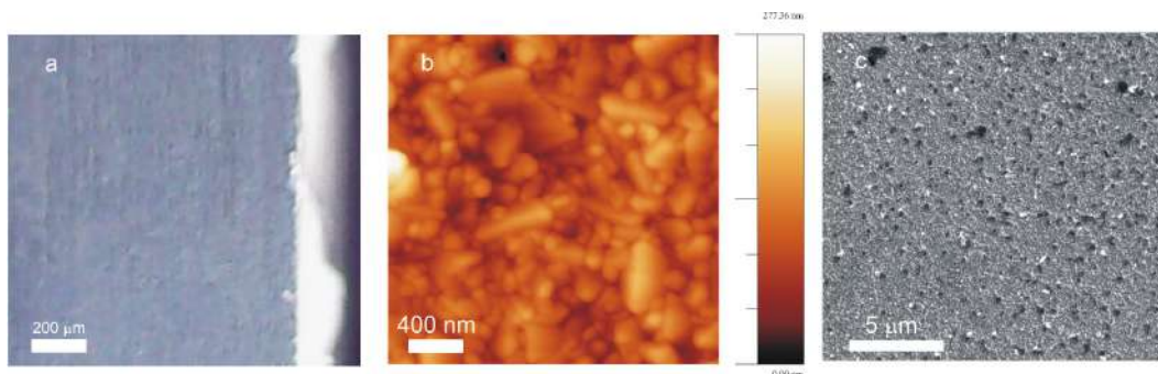
Fig. S10. a) Cross-section microscope, b) tapping mode atomic force microscope (AFM), and c) SEM images for (\text{C}_6\text{H}_5\text{CH}_2\text{NH}_3)_2\text{SnBr}_4 microcrystal film with a thickness of 155 \pm 23 \mu\text{m} . The film is prepared from the solution of microcrystals and 2 ml Poly(methyl methacrylate) (PMMA 5% concentration). The solution was spin-coated on a UV-ozone treated cover glass substrate with 500 rpm for 60 s (acceleration: 100 rpm per s).
