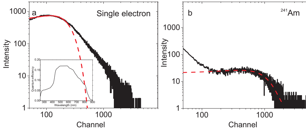
Fig. S8. a) Measured single electron response of the Hamamatsu R9880U-20 photomultiplier tube (PMT). The inset shows the quantum efficiency spectra. b) Pulse height spectra under gamma-ray excitation of ^{241}\text{Am} source at 59.5 keV. The photoelectron yield from comparing the photo peak and the single electron response peak with their gain is 585 photoelectron/MeV. Using quantum efficiency of 0.16, the light yield is 3600 photons/MeV. The energy resolution is 79.40%.
