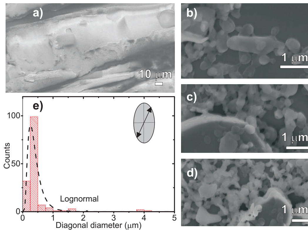
Fig. S9. (\text{C}_6\text{H}_5\text{CH}_2\text{NH}_3)_2\text{SnBr}_4 microcrystals and their size distribution. a) Scanning electron microscope (SEM) image of the surface of single crystals showing relatively smooth surfaces of the crystals. b, c, d) SEM images of the microcrystals after the ultrasonic bath. e) Sizes of the microcrystals with their lognormal distribution.
