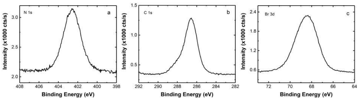
Fig. S3. XPS spectra of a) N 1s, b) C 1s and c) Br 3d of (\text{C}_6\text{H}_5\text{CH}_2\text{NH}_3)_2\text{SnBr}_4 .
