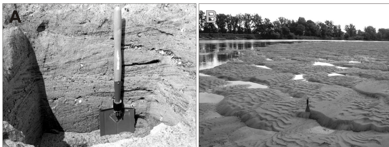
Fig. 5. The Ciechocinek bar: A – trough cross-stratification sand and gravel in the shallow excavation (length of the spade 55 cm); B – transversal chain megaripples (after Allen 1968) with superimposed small ripples (length of the spatula – 25 cm)
