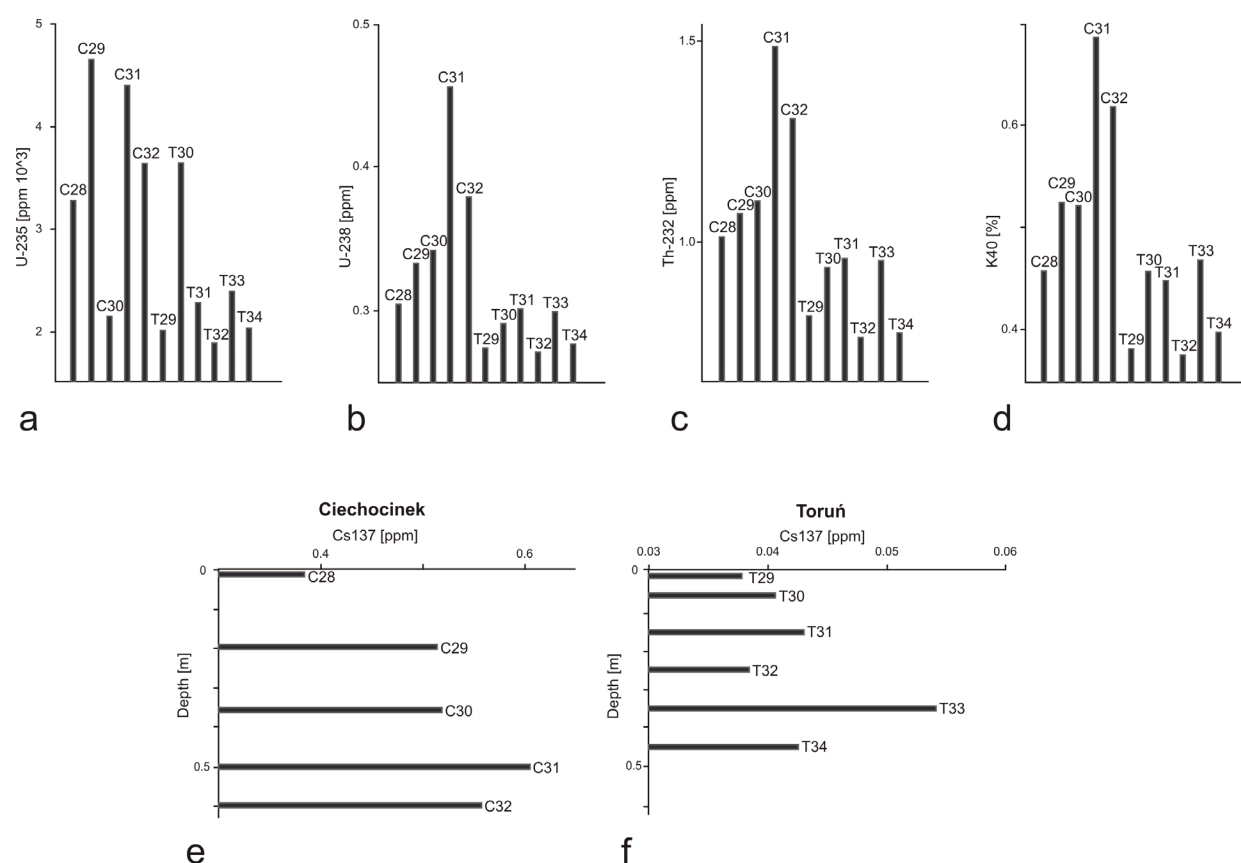
Fig 9. Concentration of radioisotopes measured by gamma spectrometry for bar sediment samples: a – ^{235}\text{U} , b – ^{238}\text{U} , c – ^{232}\text{Th} , d – ^{40}\text{K} and dependence of ^{137}\text{Cs} concentration on depth of sample for: e – Ciechocinek site and f – Toruń site
