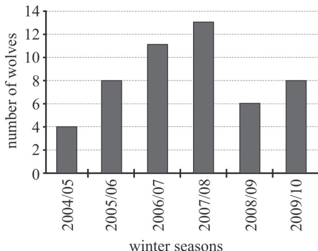
Figure 5. The estimated population dynamics (2004/2005–2009/2010) of wolves in the Bydgoszcz Primeval Forest
