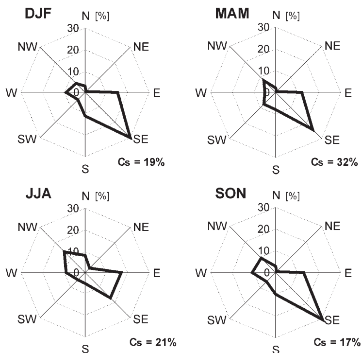
Fig. 2. Frequency of wind directions (%) and periods of calm (Cs) in Ny Ålesund in the period 1975–1989 (Hanssen-Bauer et al. 1990).
