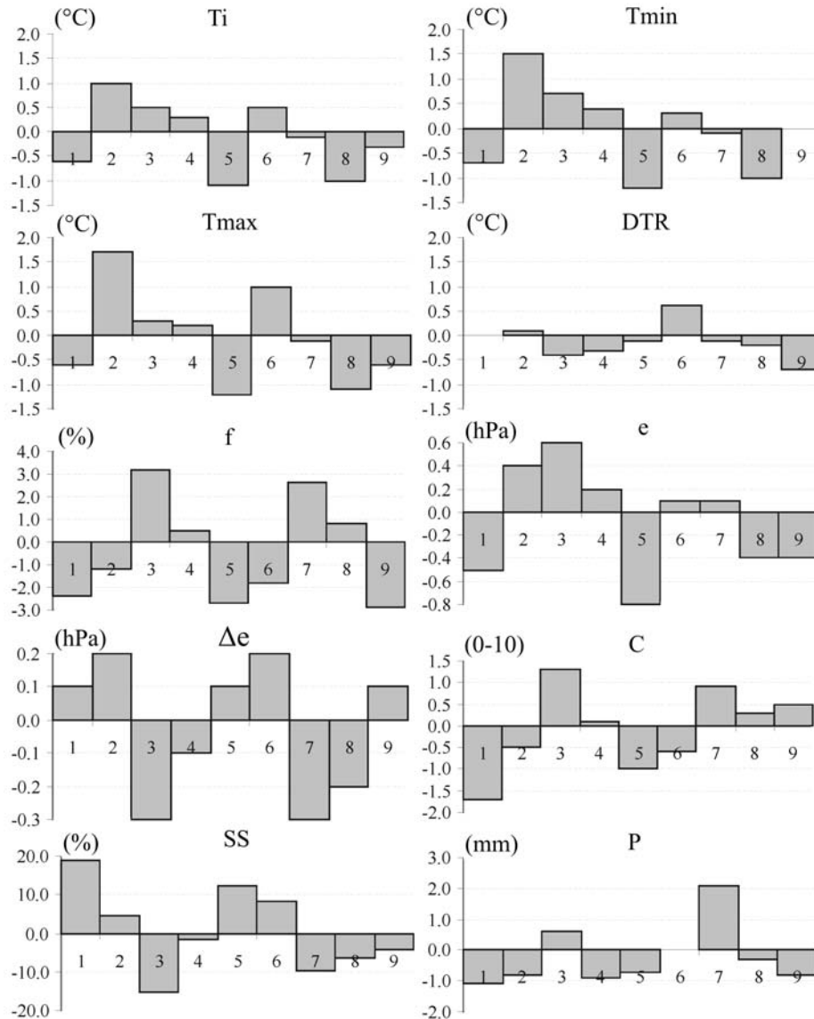
Fig. 6. Mean anomalies of selected meteorological elements for particular types of circulation in the Kaffiöyra Plain in the period July 21 st – August 31 st , 1975–2000 (Przybylak et al. 2004). Types of circulation: 1 NWa+Na+NEa; 2 Ea+SEa; 3 Sa+SWa+Wa; 4 Ca+Ka; 5 NWc+Nc+NEc; 6 Ec+SEc; 7 Sc+SWc+Wc; 8 Cc+Bc; 9 X. Remaining abbreviations as in Tables 1 and 2.
