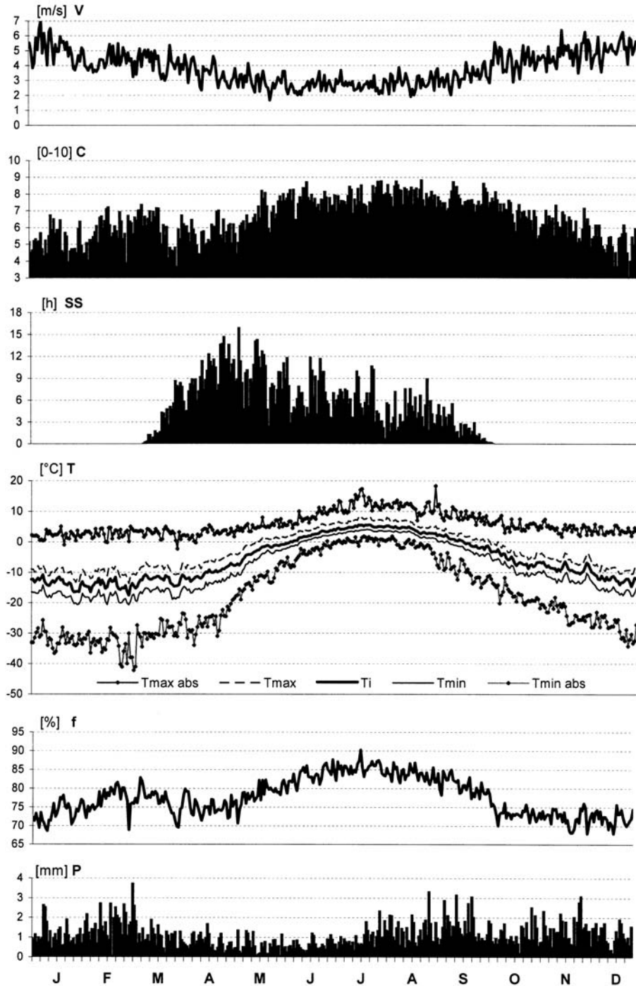
Fig. 3. Mean annual courses of selected meteorological elements in Ny Ålesund during the period 1975–2000 according to daily values. Key to abbreviations as in Table 1.
