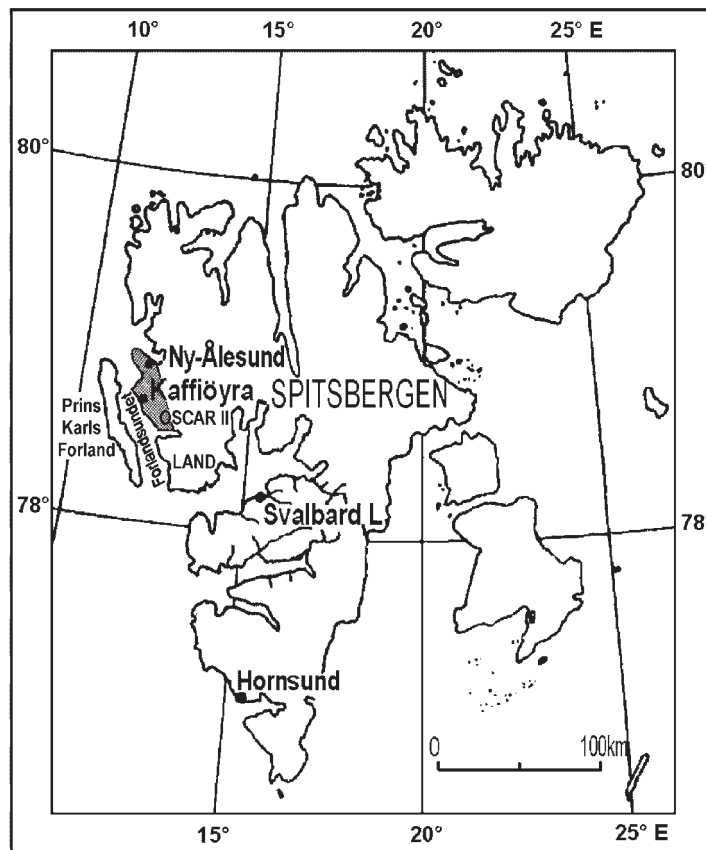
Fig. 1. Location of research area (in grey) and meteorological stations used in the study.
