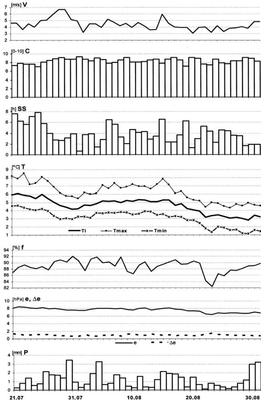
Fig. 5. Course of meteorological elements on the Kaffiöyra Plain in the summer season (July 21 st – August 31 st ), 1975–2000. Remaining abbreviations as in Tables 1 and 2.
