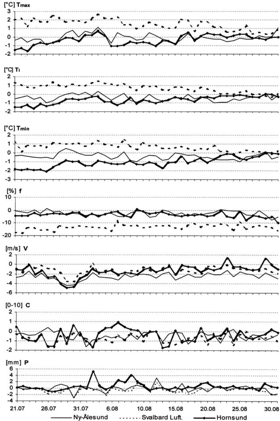
Fig. 7. Course of differences of mean values of selected meteorological elements in the summer season (July 21 st – August 31 st ) between the Kaffiöyra-Heggodden station and other analysed Spitsbergen stations, 1975–2000. Abbreviations as in Table 1.
