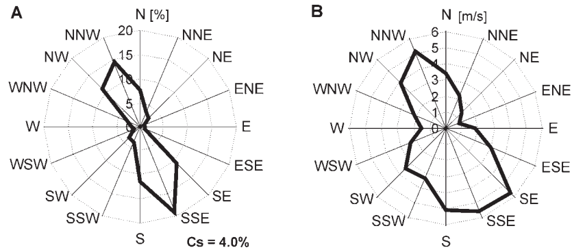
Fig. 4. A. Frequency of wind directions (%) and periods of calm (Cs) and B mean wind velocities (m/s) according to direction on the Kaffiöyra Plain in the summer season (July 21 st – August 31 st ), 1975–2000
