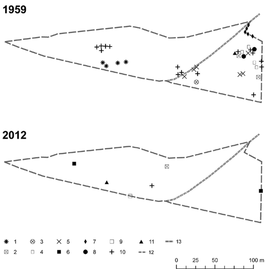
Figure 7. Spatio-temporal changes in the location of selected plant species in 1959 and 2012. Explanations of symbols: 1 – Anemone sylvestris , 2 – Inula hirta , 3 – Iris sibirica , 4 – Linum catharticum , 5 – Linum perenne , 6 – Peucedanum cervaria , 7 – Pulmonaria angustifolia , 8 – Scabiosa canescens , 9 – Seseli minima , 10 – Stipa joannis , 11 – Thesium linophyllon , 12 – boundary of the study area, 13 – road
