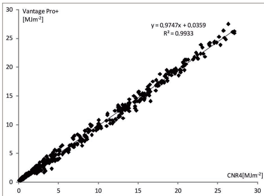
Fig. 5. Relation between mean diurnal sums of global solar radiation obtained by the CNR4 and the Vantage Pro+ instruments at the OME point in 2012
