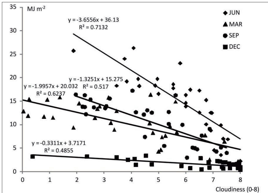
Fig. 10. Relation between diurnal values of cloudiness (WRZ) and global solar radiation in OME in March (MAR), June (JUN), September (SEP) and December (DEC) 2012
