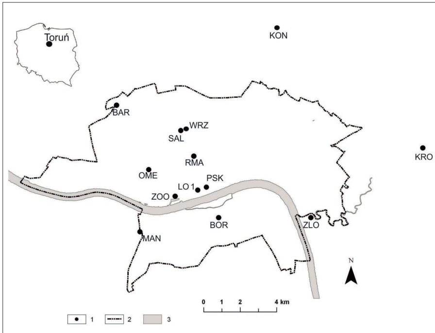
Fig. 1. Measurement points used for the observation of global solar radiation in Toruń and its suburbs in 2012: 1 – Measurement points; 2 – Administrative boundary of the city; 3 – The Vistula River
