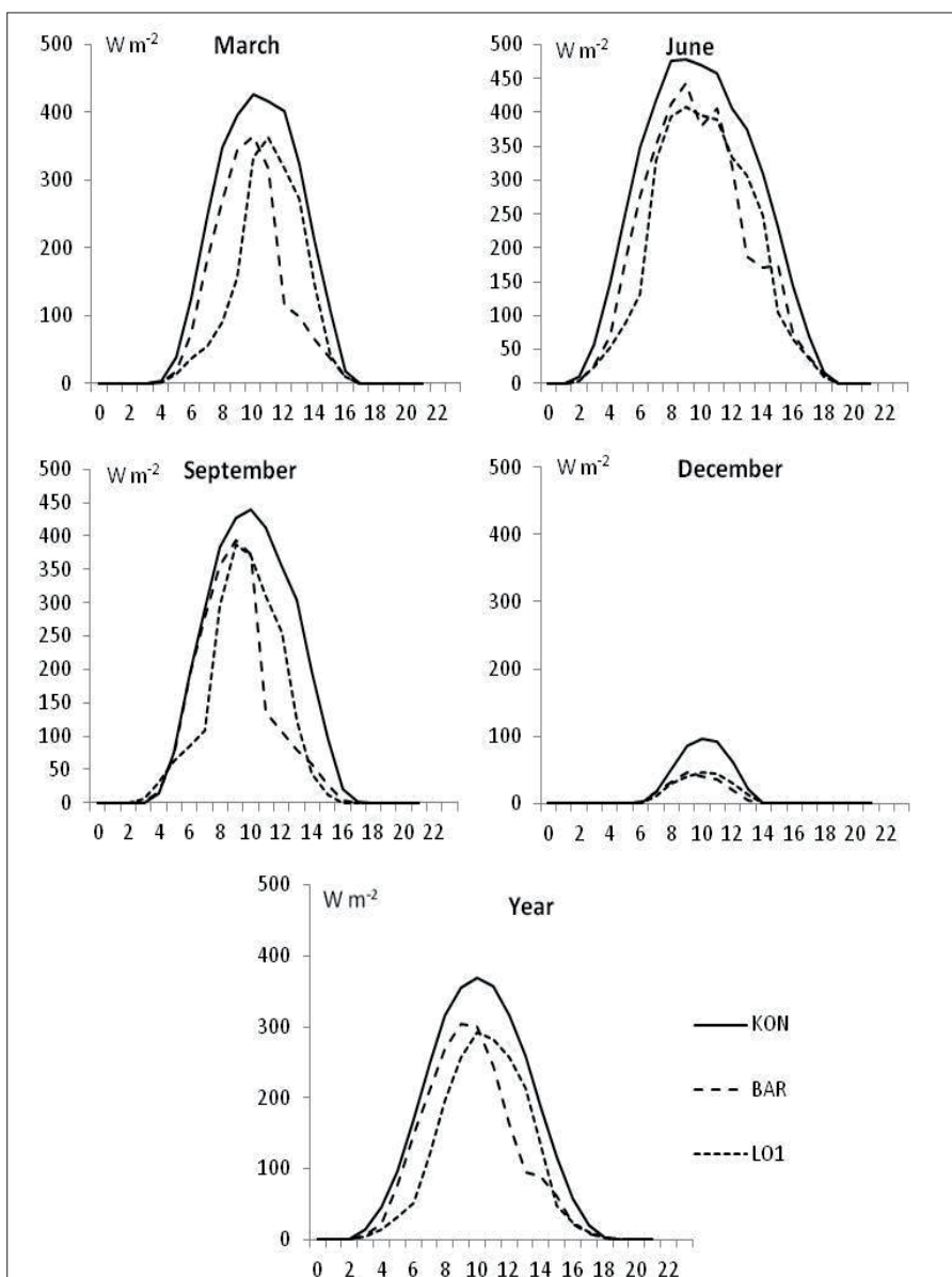
Fig. 11. Daily course of solar global radiation in selected months and year at KON, BAR and LO1 in 2012 (zonal time)
