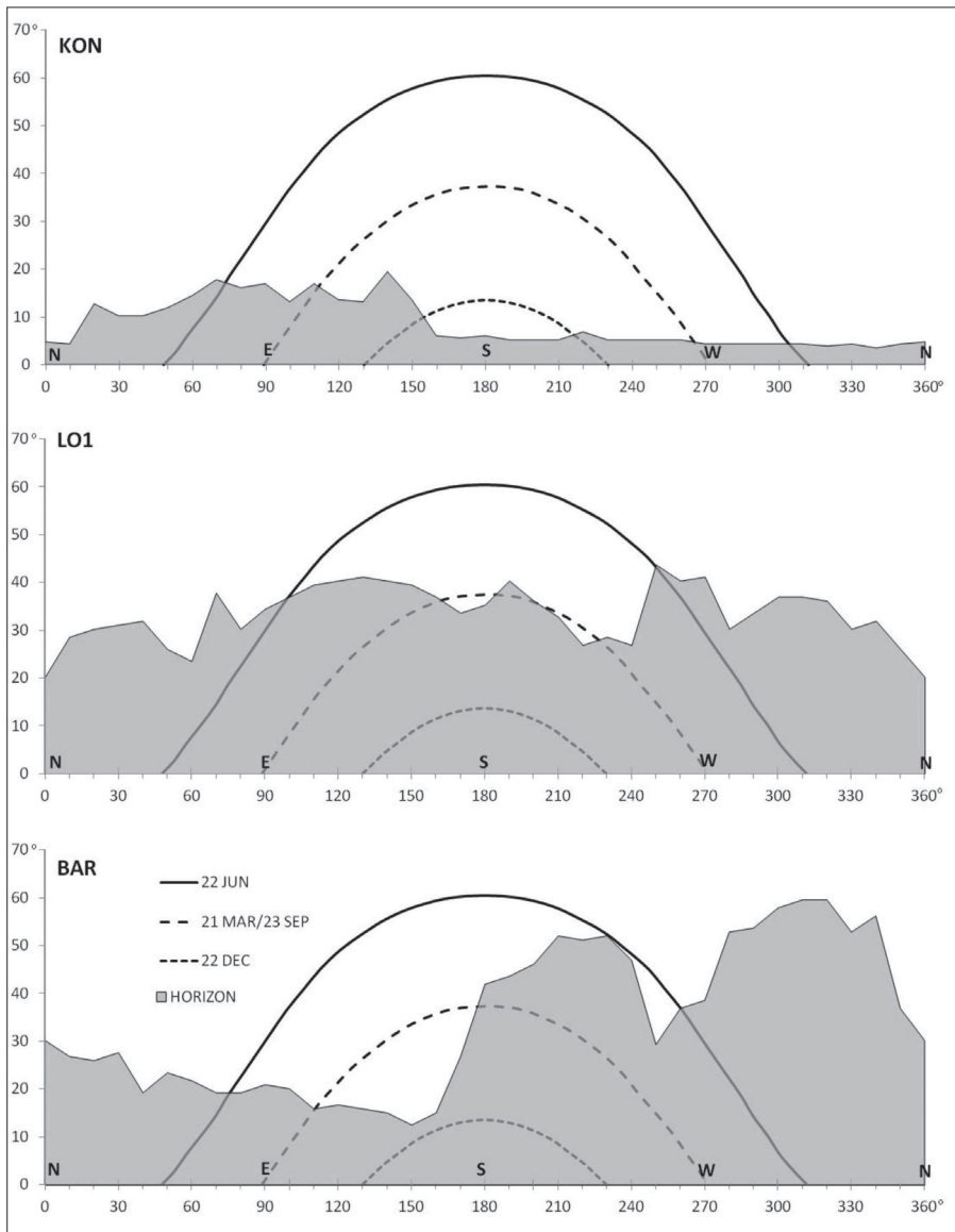
Fig. 3. The obstruction of the horizon at the KON, BAR and LO1 points, and the sun's path on 21 March/23 September, and on 22 June and 22 December
