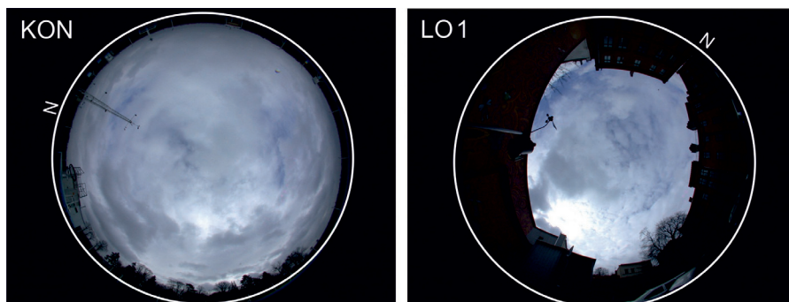
Fig. 2. The obstruction of the horizon at the KON and LO1 points (photo by Marcin Rzepa)
