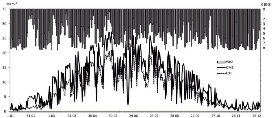
Fig. 9. Annual course of cloudiness (C) in Toruń (WRZ) and solar global radiation at the OME and LO1 in 2012
