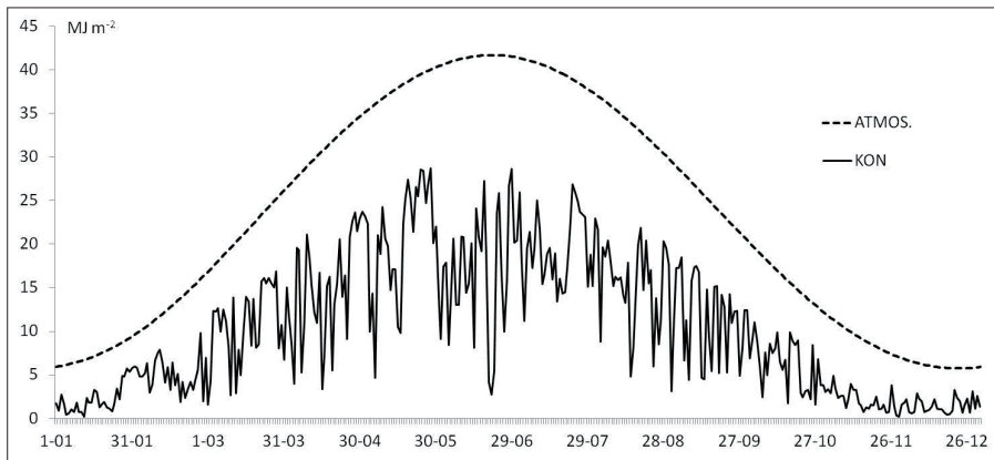
Fig. 6. The annual course of daily sums of global extraterrestrial solar radiation, 53°N (ATMOS), and at KON in 2012
