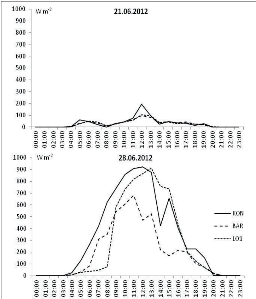
Fig. 12. Daily course of solar global radiation at KON, BAR and LO1 in 21 and 28 June, 2012 (zonal time)
