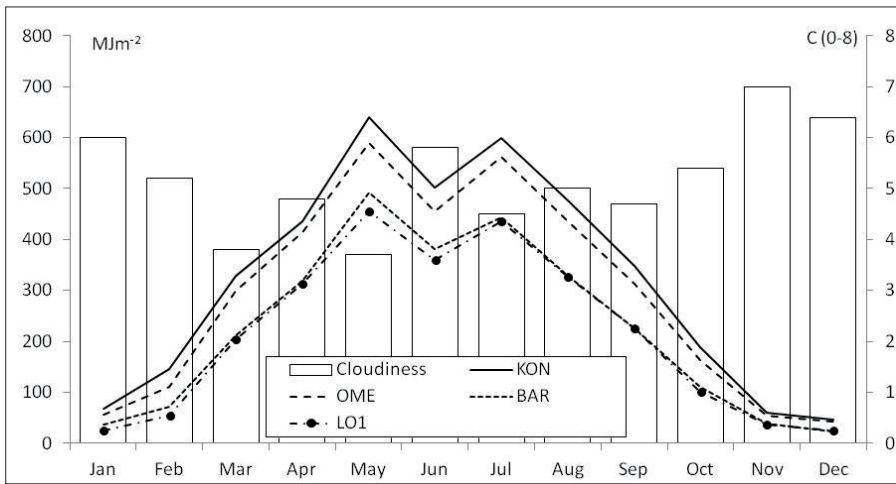
Fig. 7. Course of monthly sums of global solar radiation ( \text{MJm}^{-2} ) at selected stands and cloudiness (C on a scale of 0–8) in Toruń in 2012
