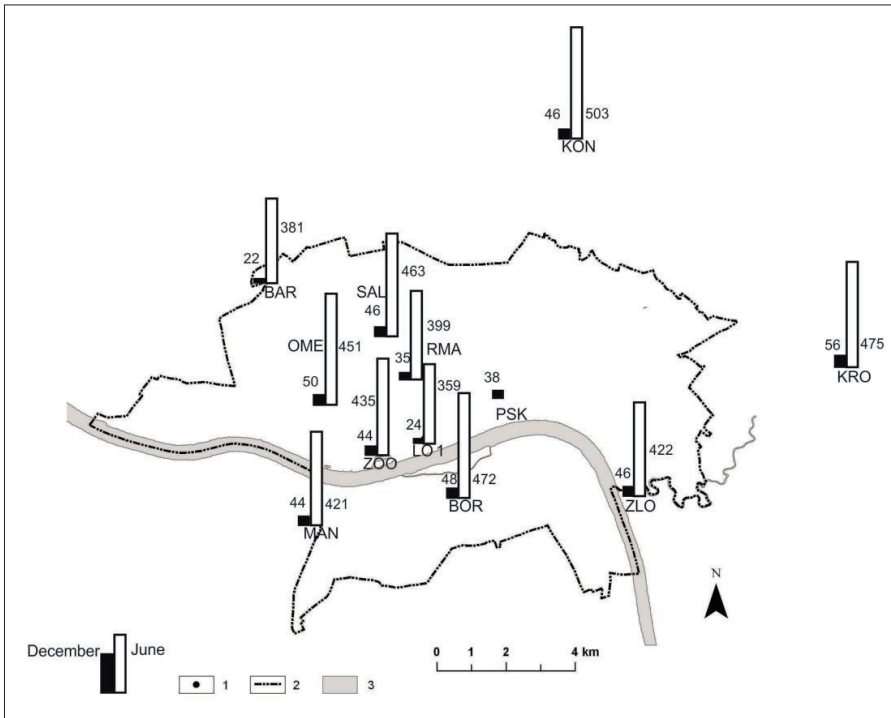
Fig. 8. Monthly sums of solar radiation (in MJ·m -2 ) in Toruń and its suburbs in June and December 2012: 1 – Measurement points; 2 – Administrative boundary of the city; 3 – The Vistula River
