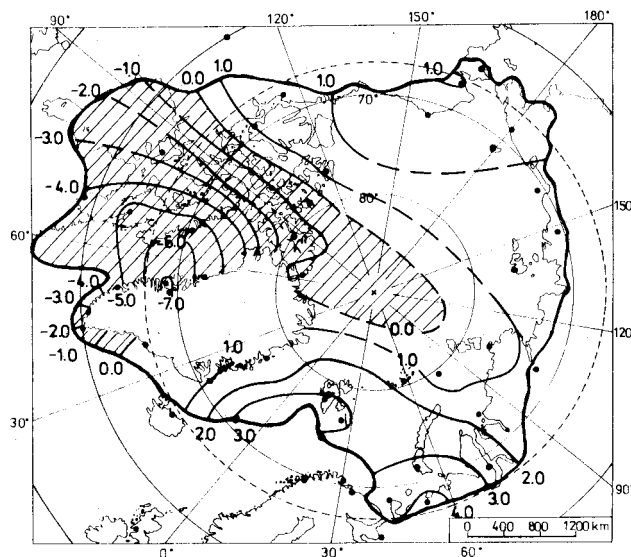
Figure 12. Differences of air temperature (in °C) between the most extreme 7-year run of NAO+ winters (December–February 1989–1995) and NAO- winters (December–February 1963–1969). The NAO+ and NAO- winters were taken after Dickson et al. (1997). Negative differences are hatched. Other key as in Figure 7
