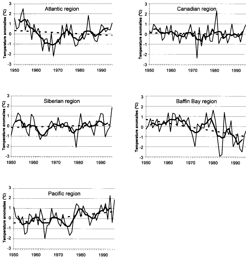
Figure 6. Year-to-year courses of mean annual anomalies of air temperature and their trends in the climatic regions of the Arctic over the period 1950–1995 (based on data from stations). Key: solid lines = year-to-year courses, heavy solid lines = running 5-year mean, and dashed lines = linear trends
