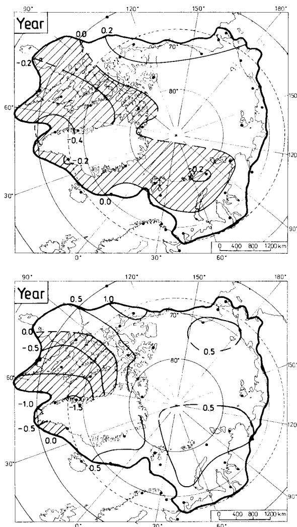
Figure 7. Spatial distribution of the mean annual air temperature trends ( ^{\circ}\text{C} per decade, upper map) over the period 1951–1995 and the anomalies of mean annual 5-year (1991–1995) air temperatures, with the 1951–1990 mean ( ^{\circ}\text{C} , lower map). Key: dashed contours over the Arctic Ocean indicate that the data are extrapolated from the coastal stations
