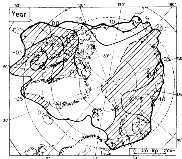
Figure 14. Differences of mean annual air temperature (in °C) between 10 years with the strongest El Niño and 10 years with the strongest La Niña phenomena. Negative differences are hatched
