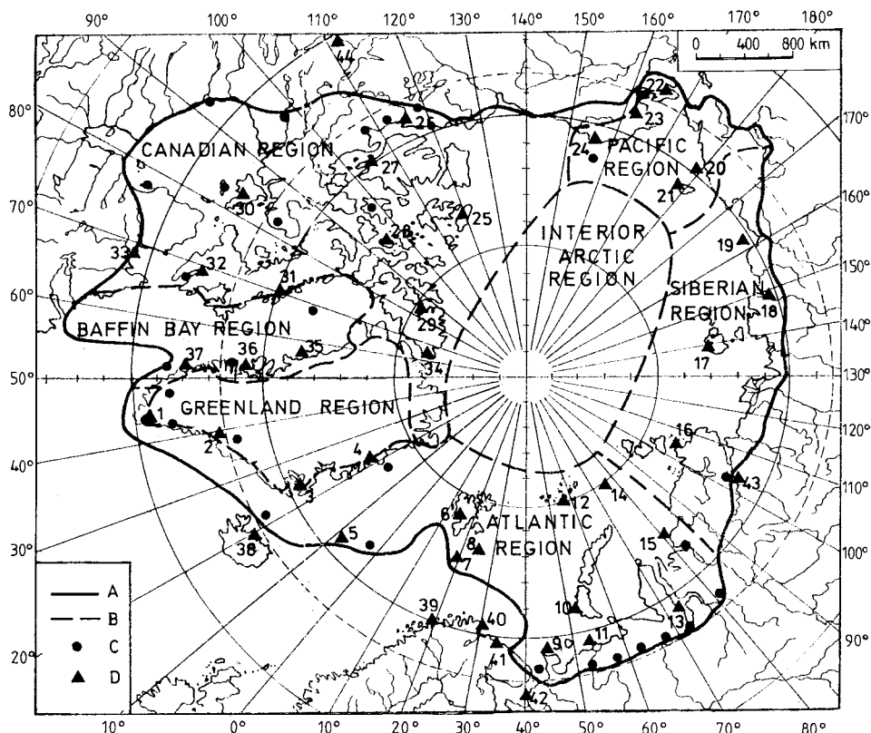
Figure 1. Location of meteorological stations and central parts of the grid-boxes used. Key—A: the border of the Arctic after Atlas Arktiki (1985); B: the borders of the climatic regions; C: central part of grid-boxes; and D: meteorological stations
