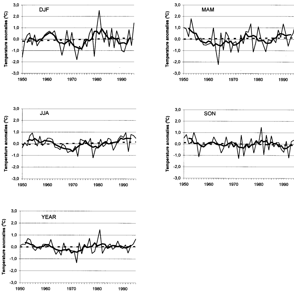
Figure 5. Year-to-year courses of mean seasonal and annual anomalies of air temperature and their trends in the Arctic over the period 1950–1995 (based on data from 30 grid-boxes after Jones, 1994, updated). Key: solid lines = year-to-year courses, heavy solid lines = running 5-year mean, and dashed lines = linear trends
