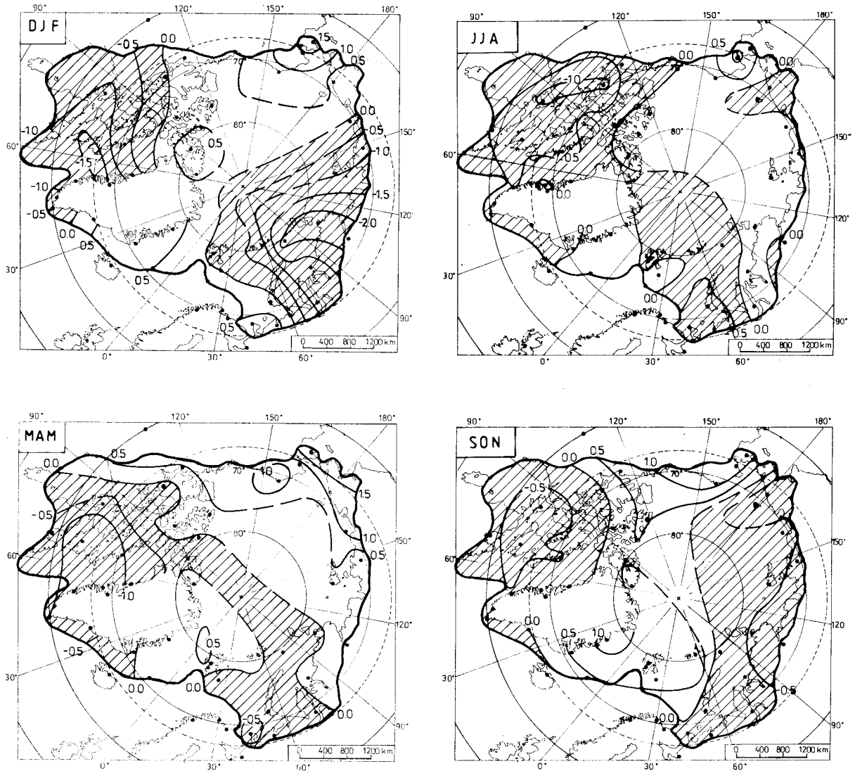
Figure 13. Differences of mean seasonal air temperature (in °C) between 10 years with the strongest El Niño and 10 years with the strongest La Niña phenomena. Negative differences are hatched. Other key as in Figure 7
