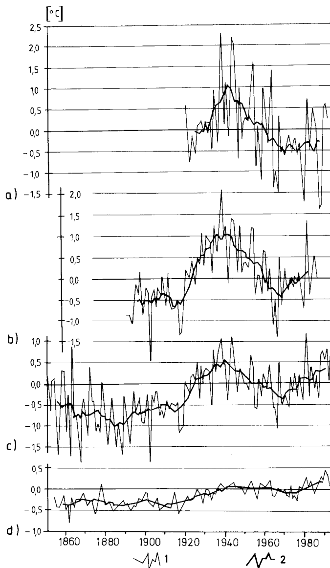
Figure 2. Year-to-year course of the annual (1, solid line) and 5-year running (2, heavy solid line) mean anomalies of air temperature for the zones (after Przybylak, 1996a): (a) 70°N–85°N (after Dmitriev, 1994); (b) 65°N–85°N (after Alekseev and Svyashchennikov, 1991); (c) 60°N–90°N (after Jones, 1995, personal communication); (d) 0°N–90°N (after Jones, 1994)
