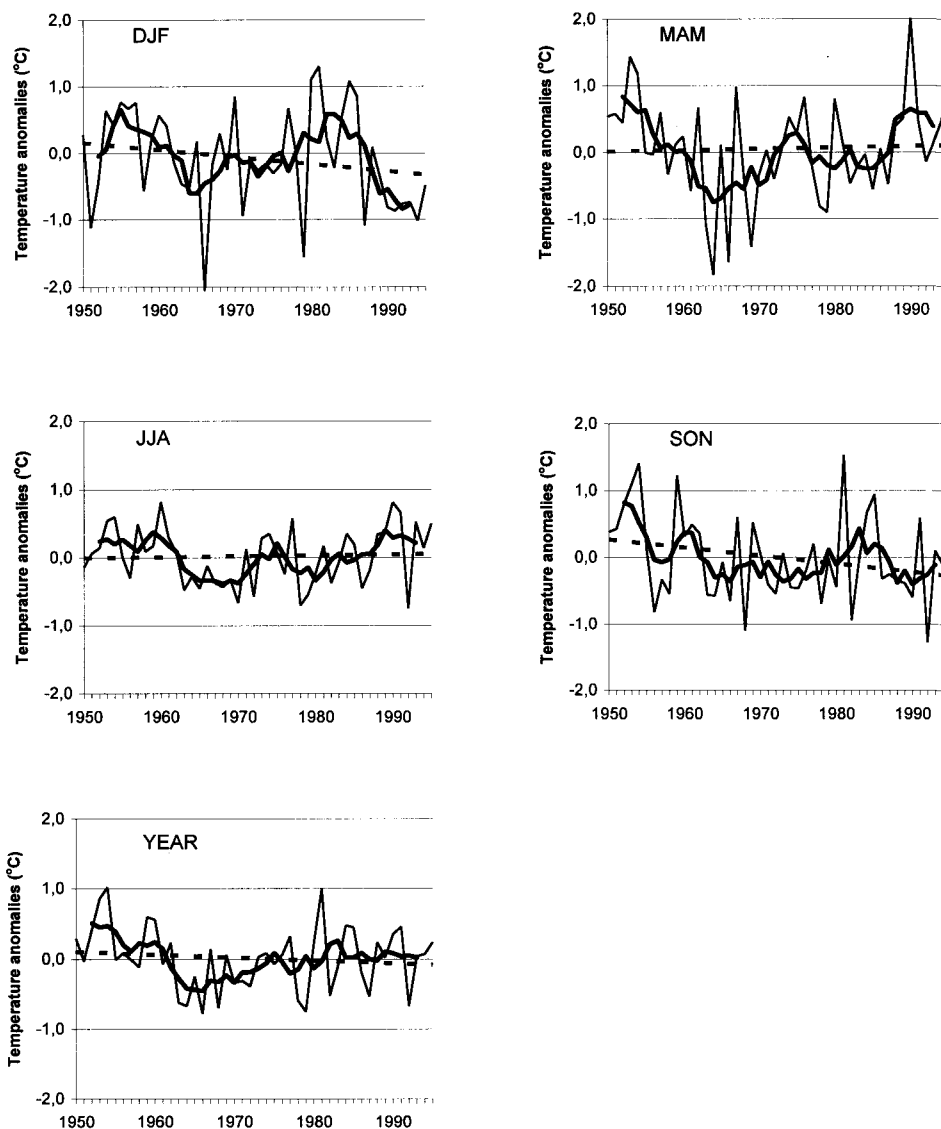
Figure 4. Year-to-year courses of mean seasonal and annual anomalies of air temperature and their trends in the Arctic over the period 1950–1995 (based on data from 33 to 35 stations). Key: solid lines = year-to-year courses, heavy solid lines = running 5-year mean, and dashed lines = linear trends
