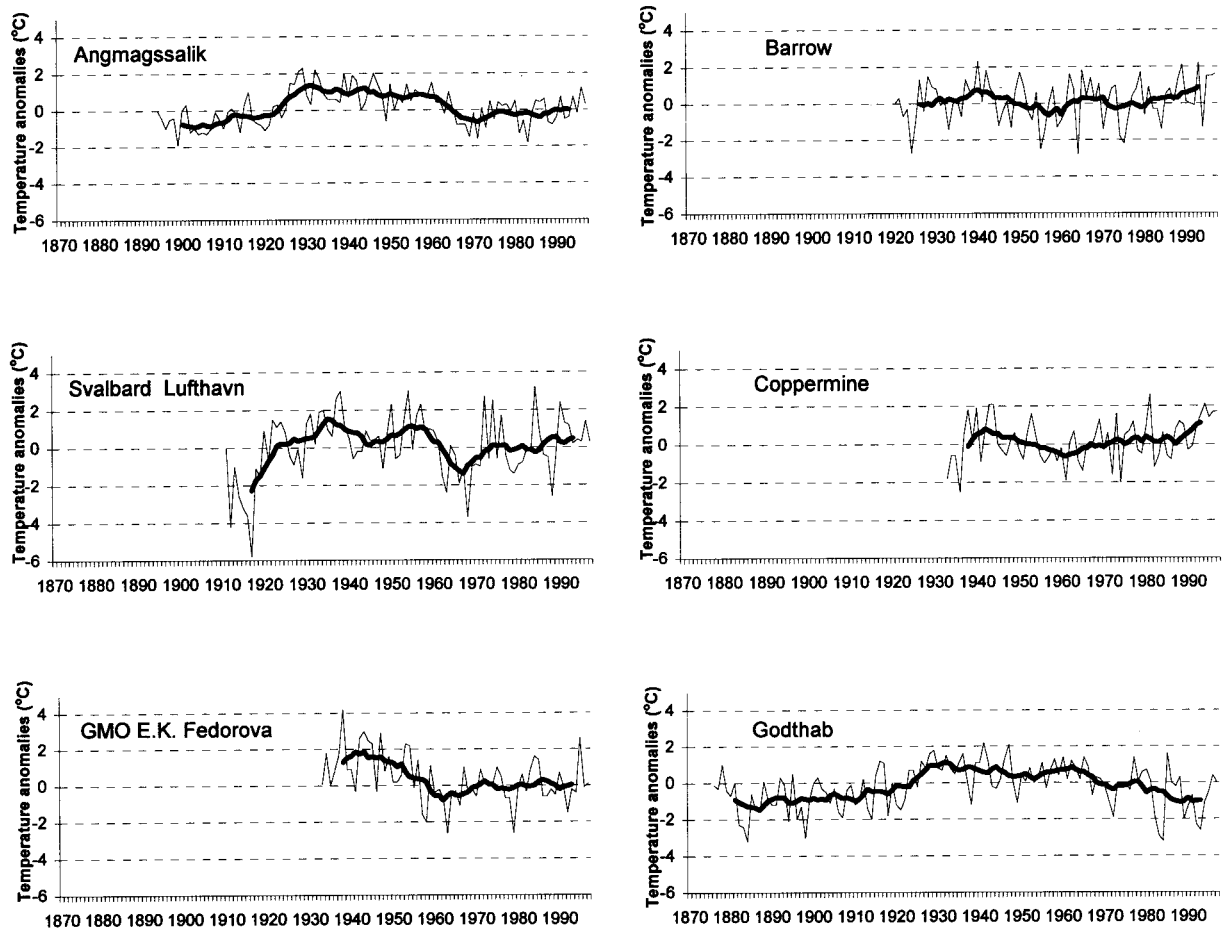
Figure 3. Year-to-year course of the annual (solid line) and 5-year running (heavy solid line) mean anomalies of air temperature in the Arctic stations having the longest observational series
