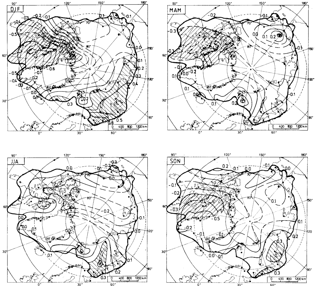
Figure 11. Spatial distribution of the coefficients of correlation between mean seasonal temperatures in the Arctic and NAOI over the period 1951–1995. Statistically significant correlations are hatched. Other key as in Figure 7
