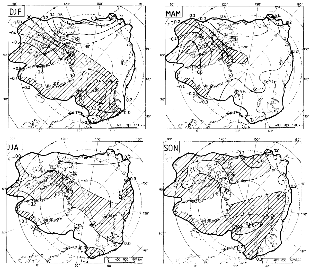
Figure 8. Spatial distribution of the mean seasonal air temperature trends ( ^{\circ}\text{C} per decade) in the Arctic over the period 1951–1995. Key as in Figure 7
