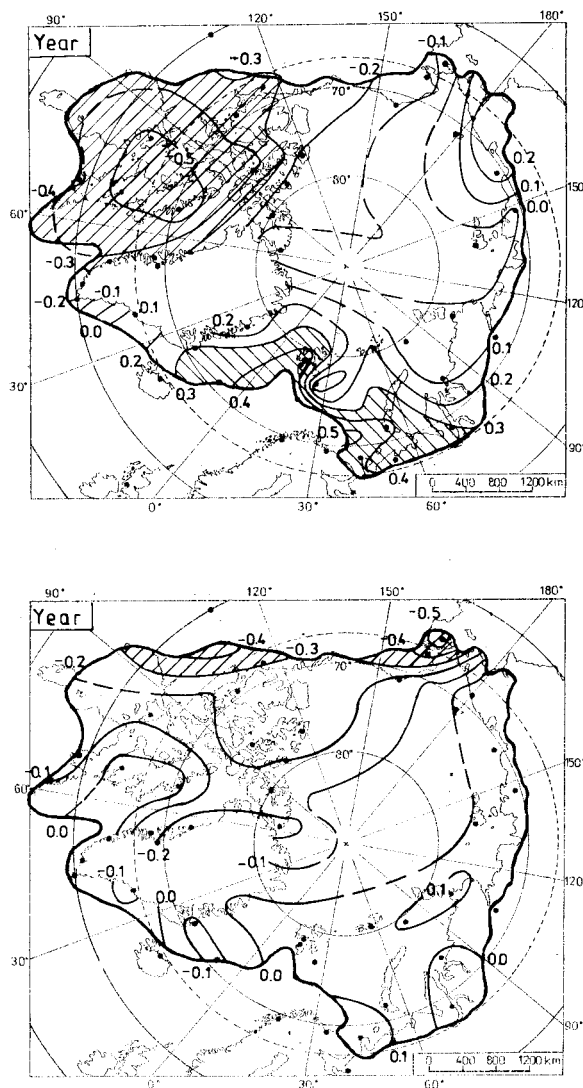
Figure 10. Spatial distribution of the coefficients of correlation between mean annual temperatures in the Arctic and NAOI (upper map) and NPI (lower map) over the period 1951–1995. Statistically significant correlations are hatched. Other key as in Figure 7
