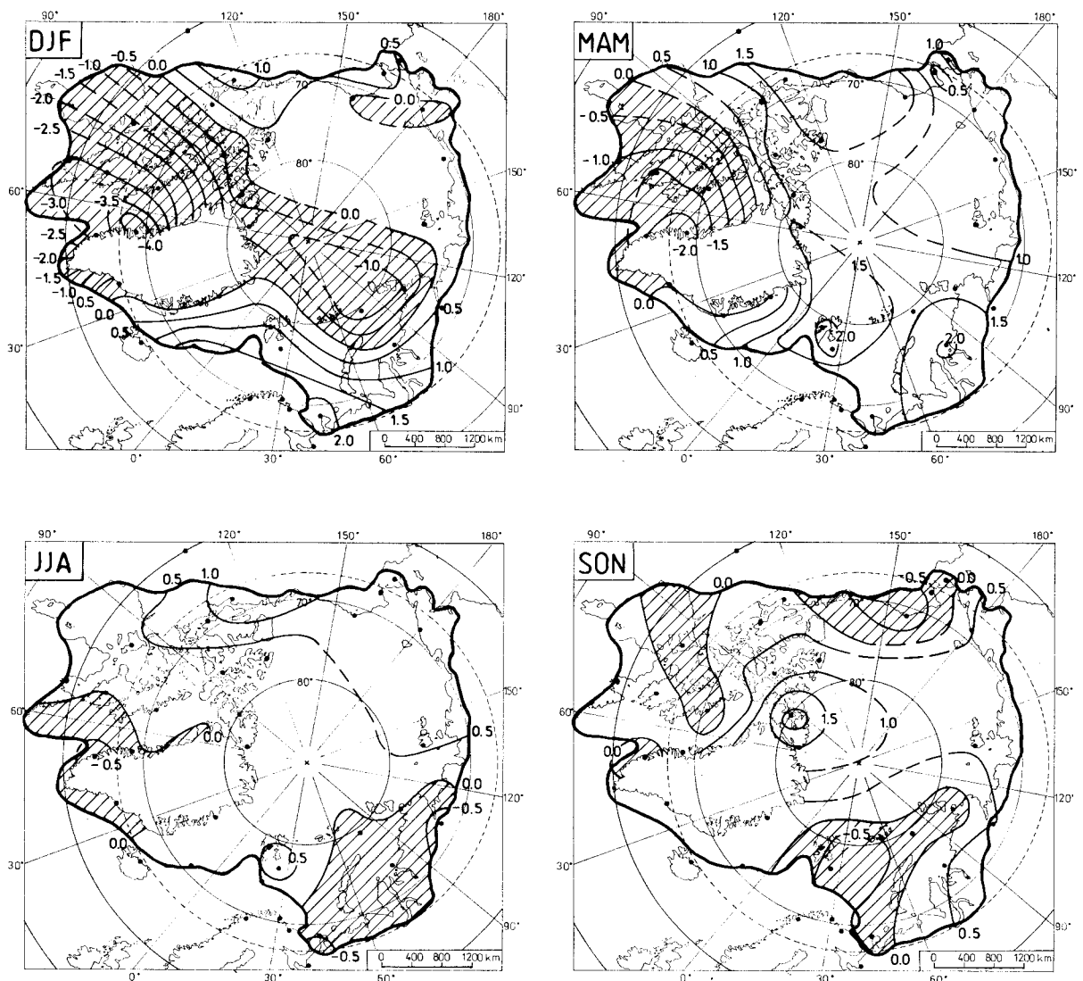
Figure 9. Spatial distribution of the anomalies of mean seasonal 5-year (1991–1995) air temperatures, with the 1951–1990 mean ( ^{\circ}\text{C} ) in the Arctic. Key as in Figure 7
