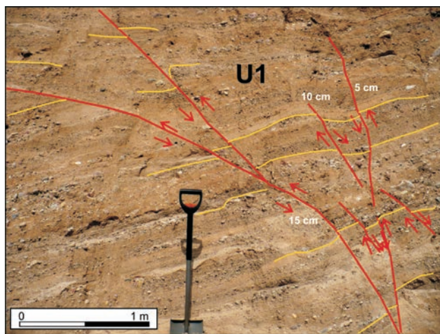
Fig. 5. Glaciotectionally disturbed sediments of the end-moraine fan at Knyszewicze.
