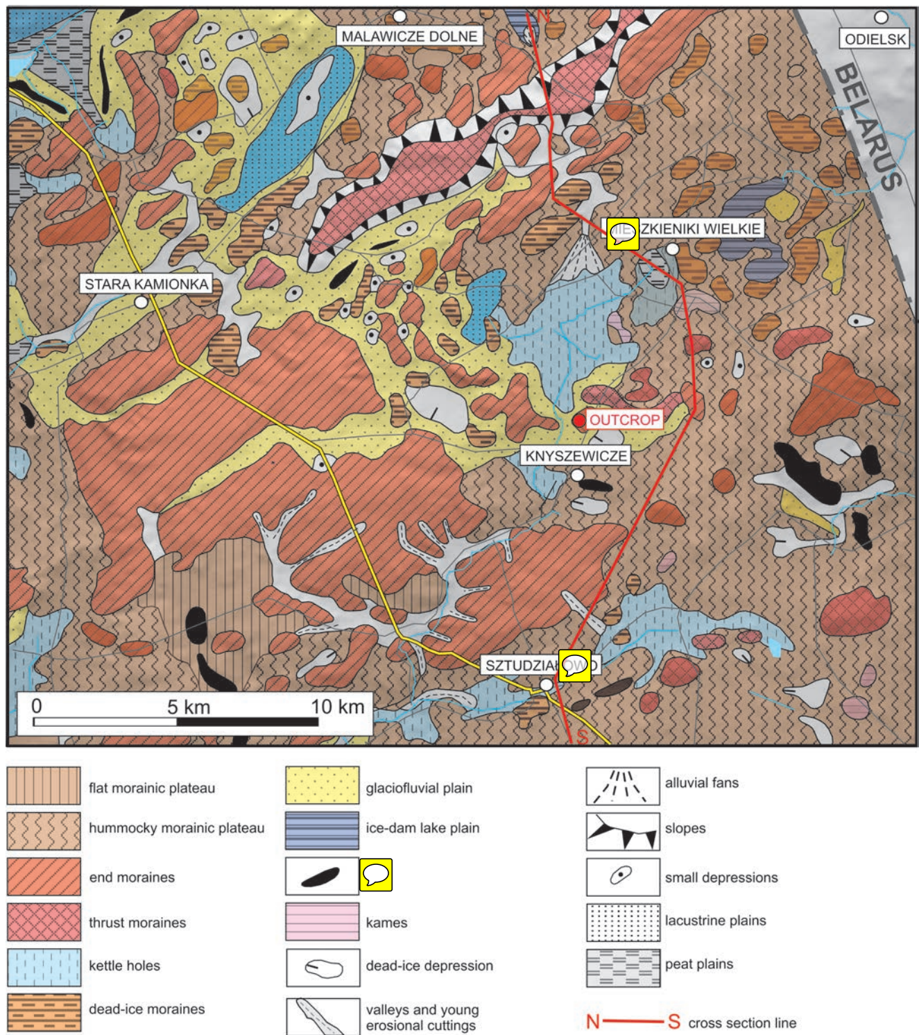
Fig. 2. Geomorphological sketch of the marginal zone of the Knyszewicze lobe (Boratyn 2003, Laskowski 2000, modified).
