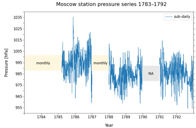
Figure 6. Station pressure series of Moscow for the period from 1783 to 1792. Shown are sub-daily values in hectopascals (blue) and shade areas that represent the availability of monthly data (yellow) or no available data (grey).
